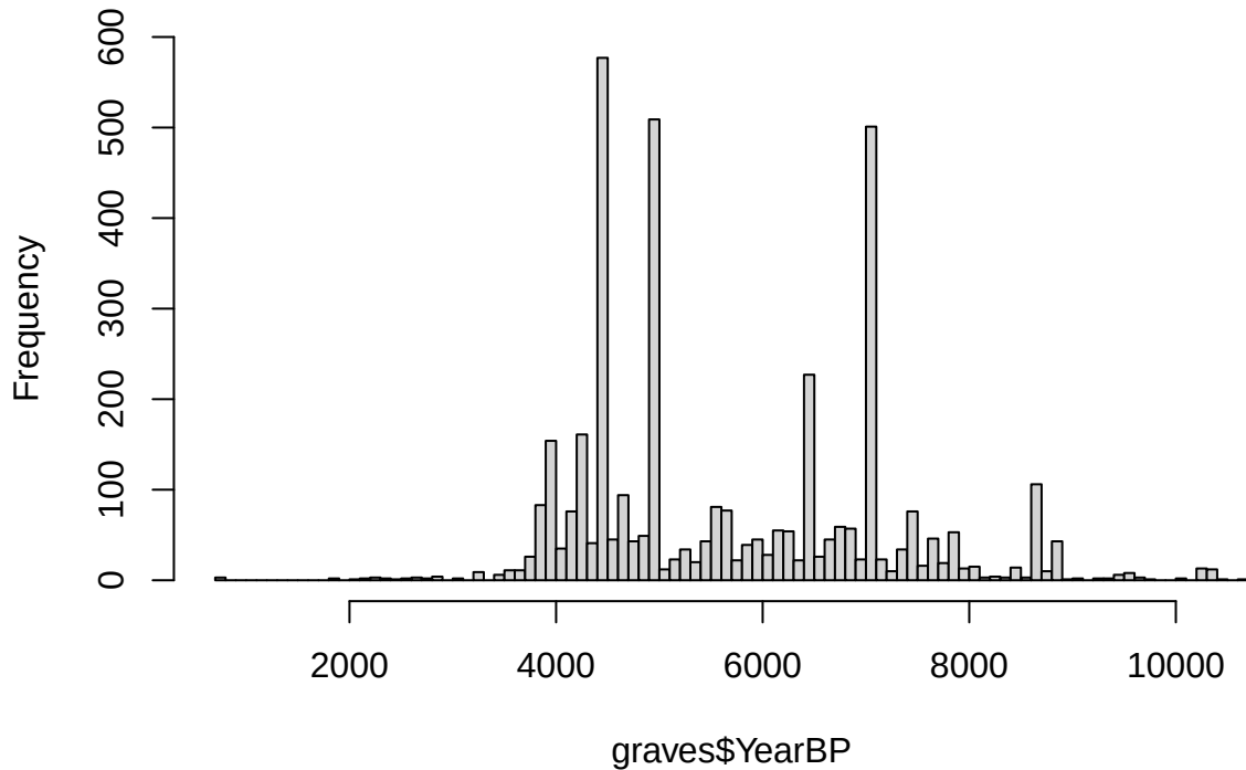
Histogram of graves$YearBP
